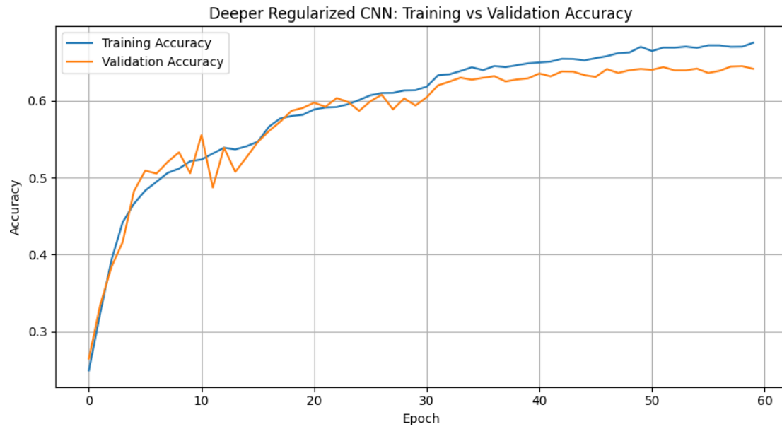
3 Figure 7: Deeper CNN training and validation accuracy.
