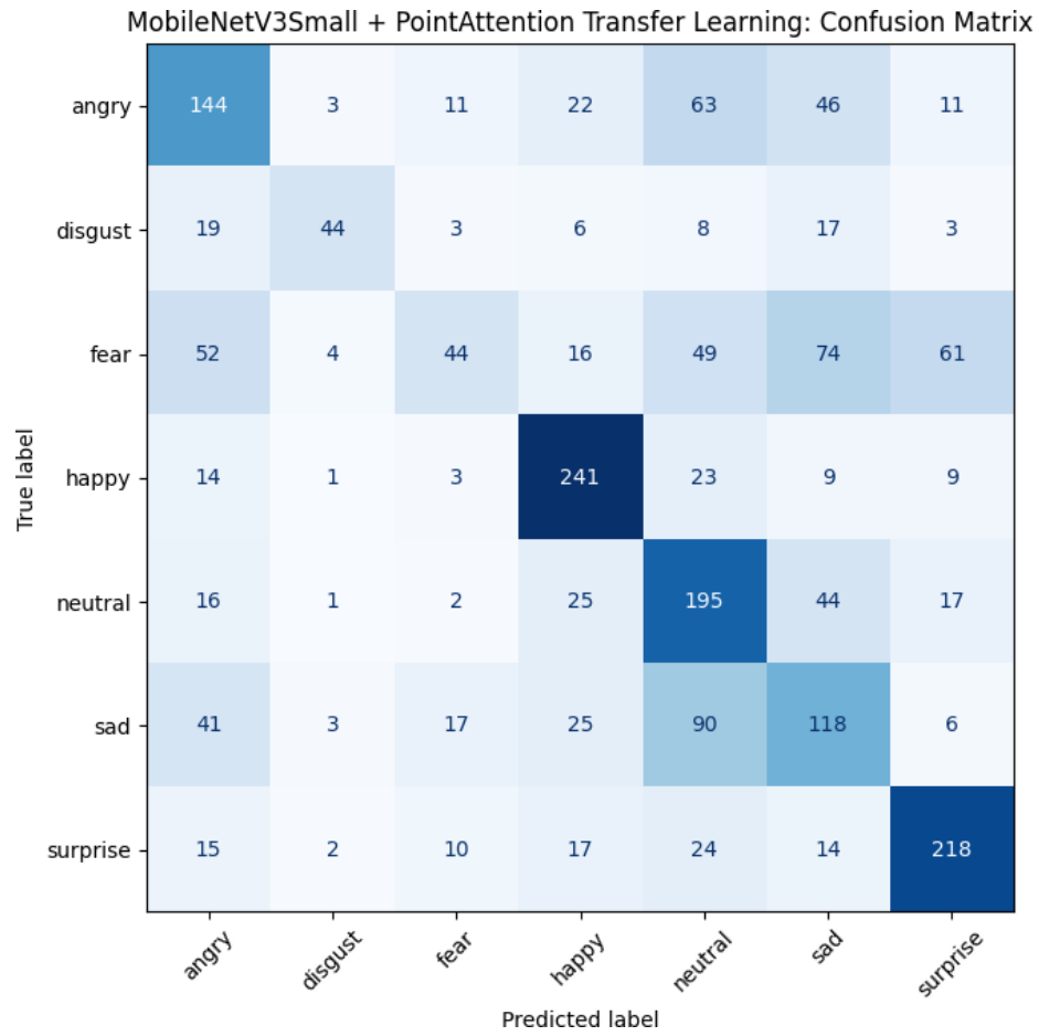
Figure 14: MobileNetV3Small + PointAttention confusion matrix.
