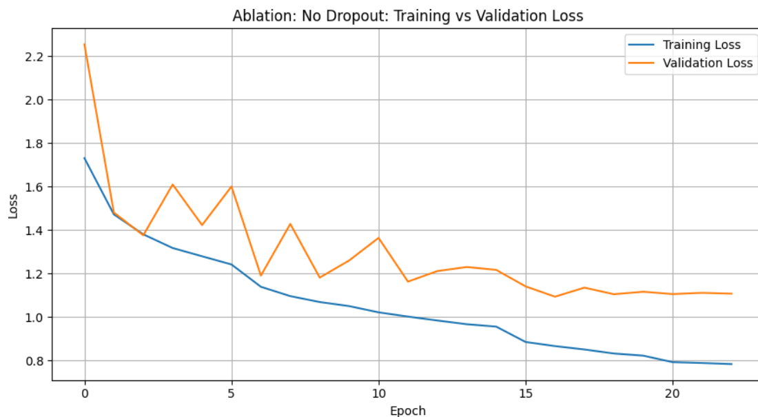
Figure 10: Ablation model training and validation loss.
