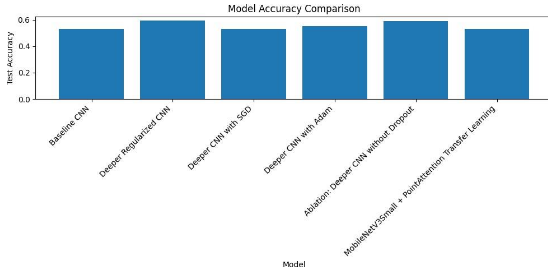
Figure 16: Model accuracy comparison.
