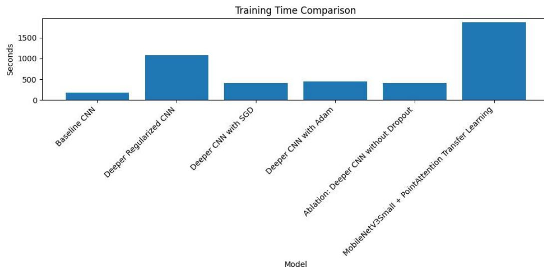
Figure 17: Training Time Comparison
